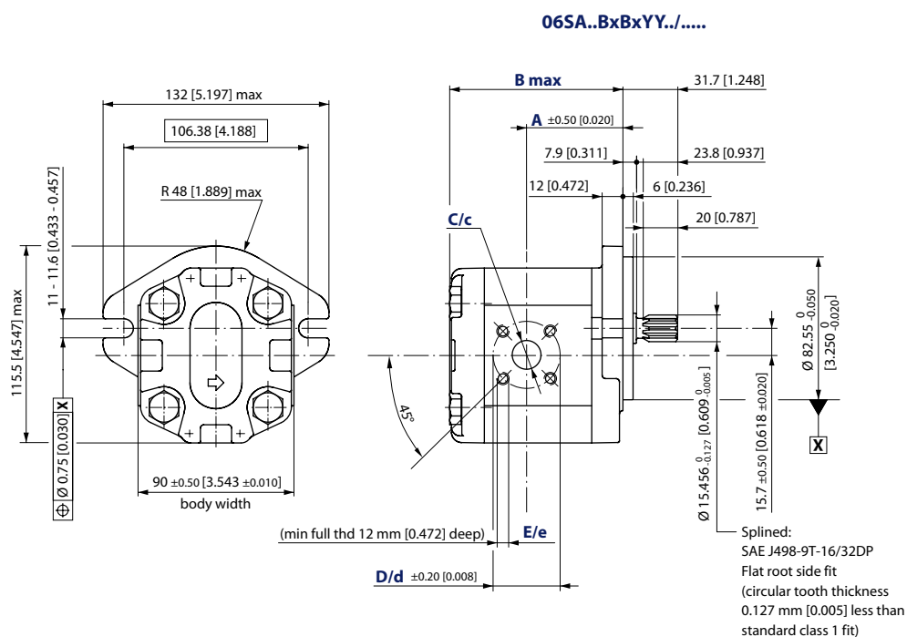
SNP2NN – 06SA..BxBxYY../..... dimensions
