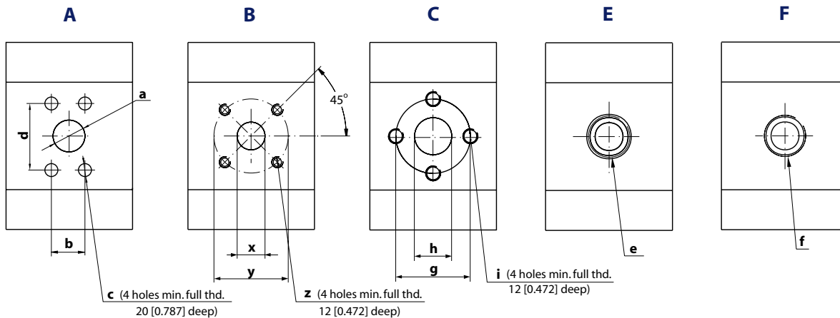
Group 3 motor ports dimensions
