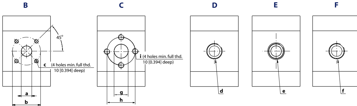
Dimensions of Group 1 pumps ports
