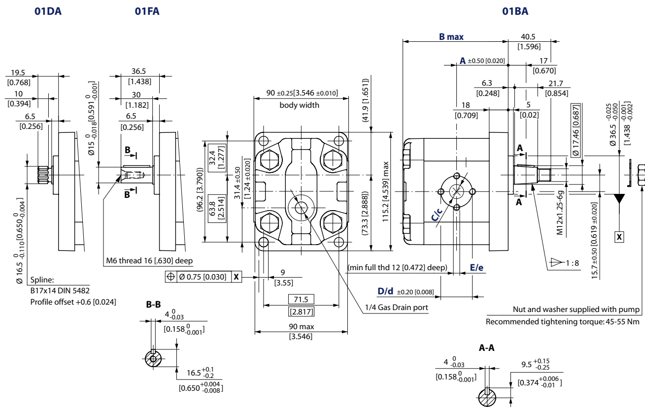
SNM2NN – 01DA, 01FA and 01BA dimensions
